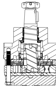
420/421 - Hydraulic Motor With Medium Duty Bearing
