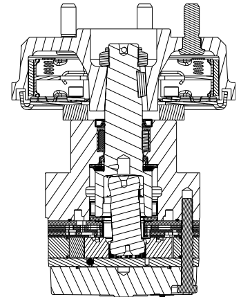
430/431 - Hydraulic Motor With Heavy Duty Bearing
